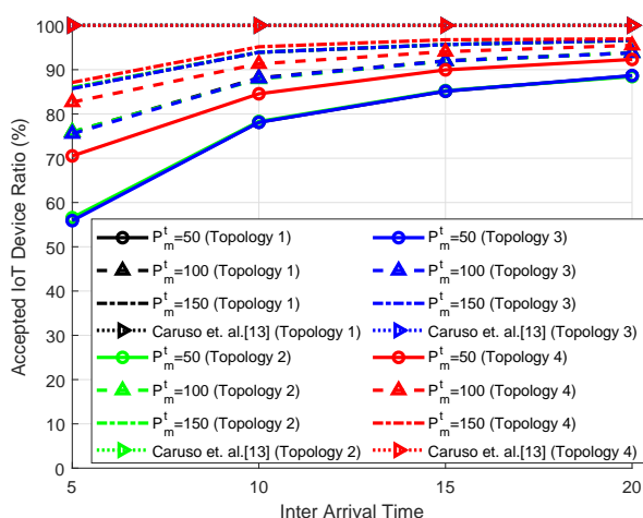
Fig. 9: Accepted IoT device ratio versus inter-arrival time in the energy harvesting environment. The scenario of the energy harvesting [13] is applied.
