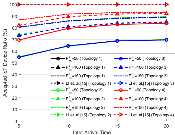
Fig. 6: Accepted IoT device ratio versus inter-arrival time.
